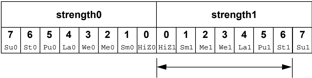
Figure 7-7—Strong H range of values
